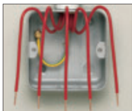
1 Install box and enter cables.
